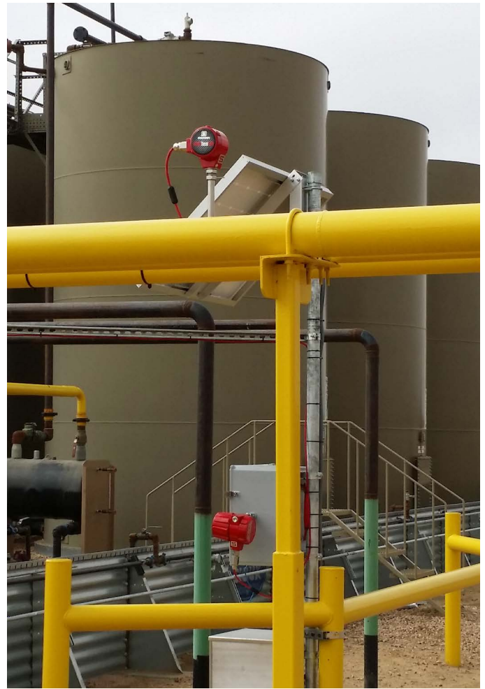
Figure 3. Flowmeters, like the QuadraTherm® 640i units shown here, measure the flow of gases at a flaring unit
