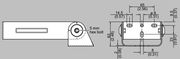
SITRANS LR150 mounting brackets, dimensions in mm (inch)
