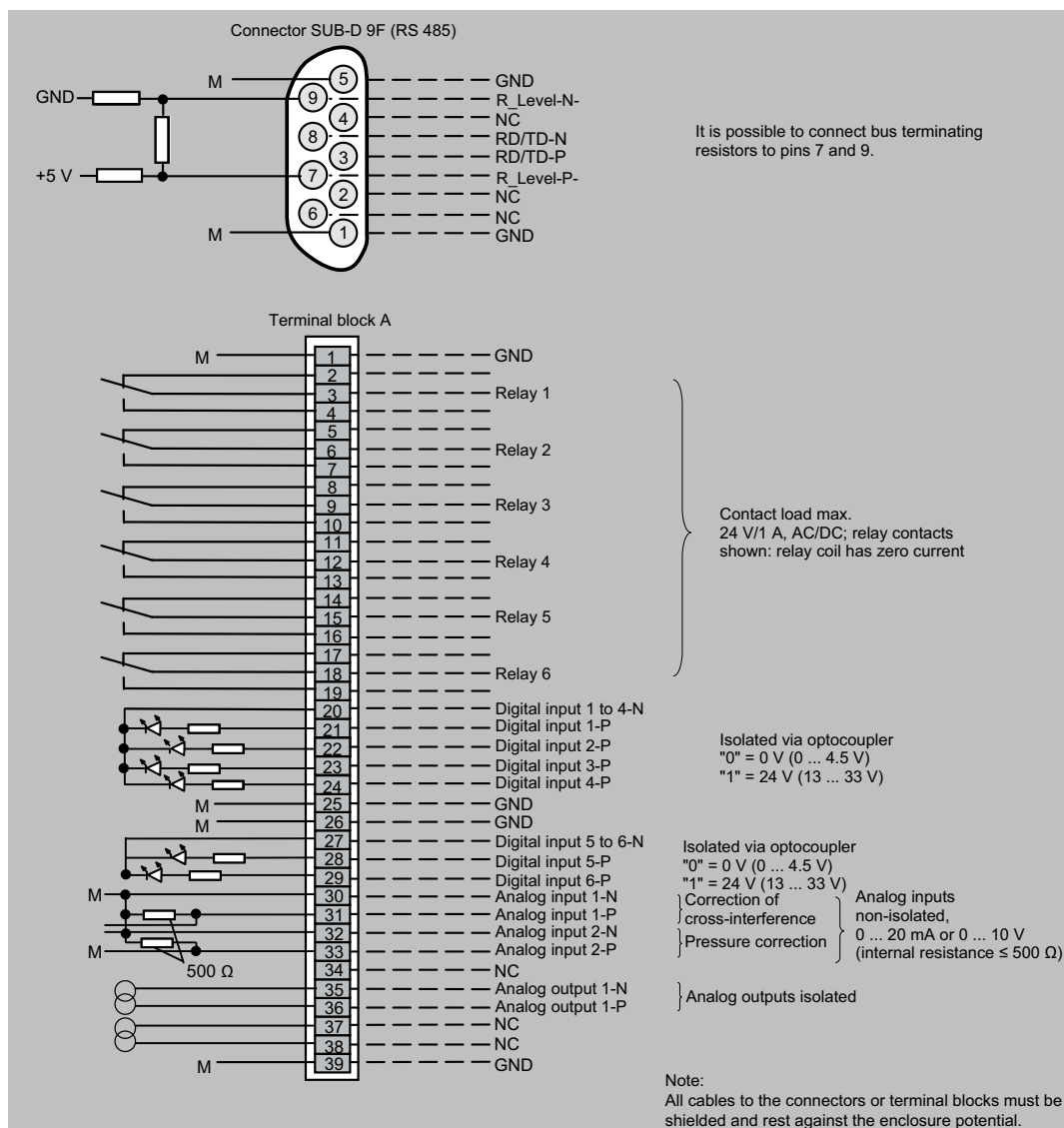
CALOMAT 62, field device, pin and terminal assignment
